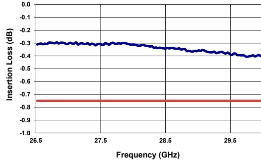
Insertion Loss ( 26.5-30 GHz )
